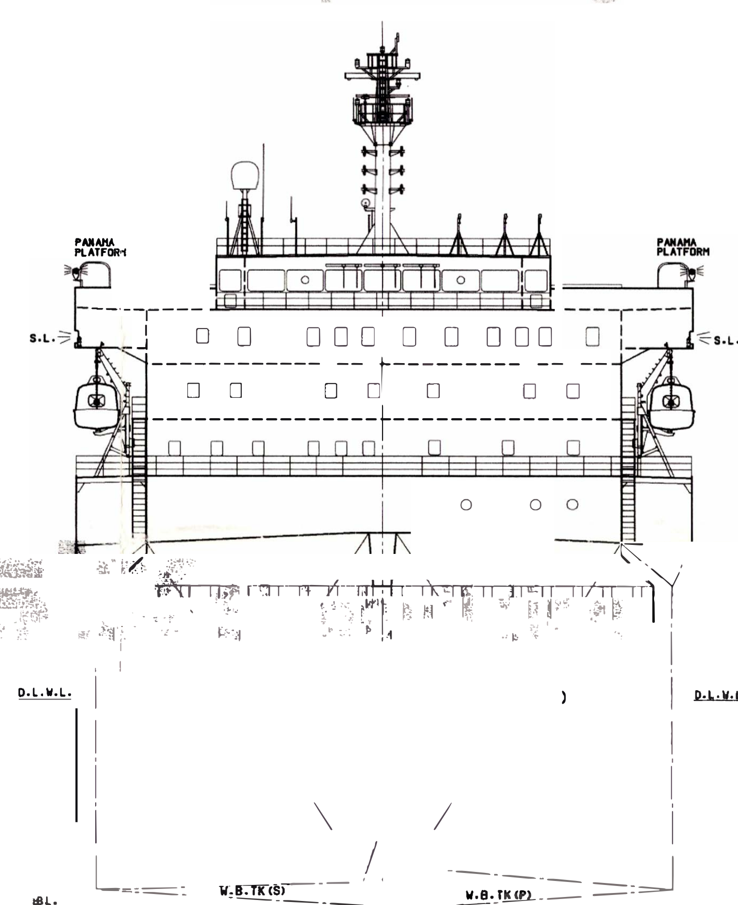
MIDSHIP SECTION
